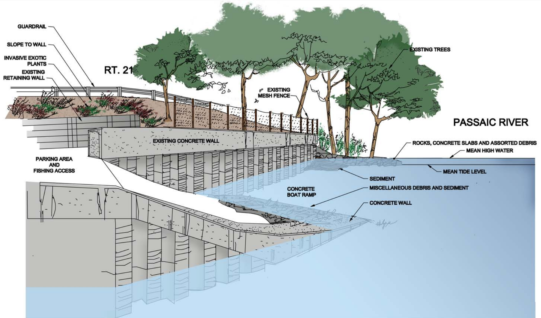
NUTLEY BOAT RAMP (BEFORE RESTORATION) NOT TO SCALE
