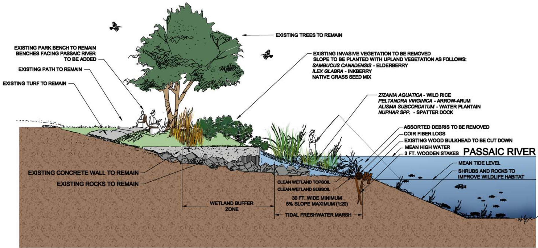
KEARNY BOAT RAMP (AFTER RESTORATION) NOT TO SCALE
